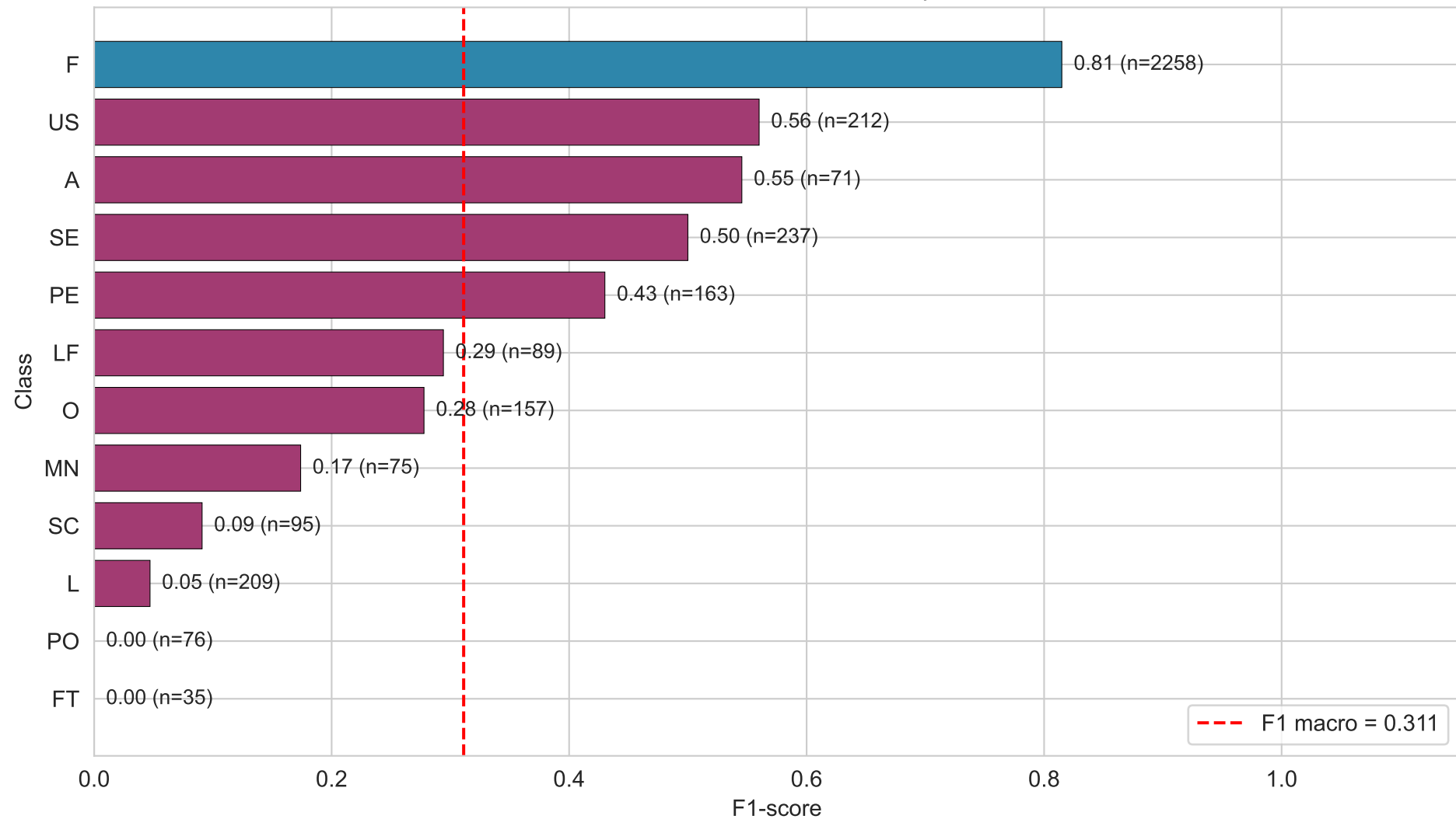
Baseline TF-IDF+LinearSVC: F1 per class
