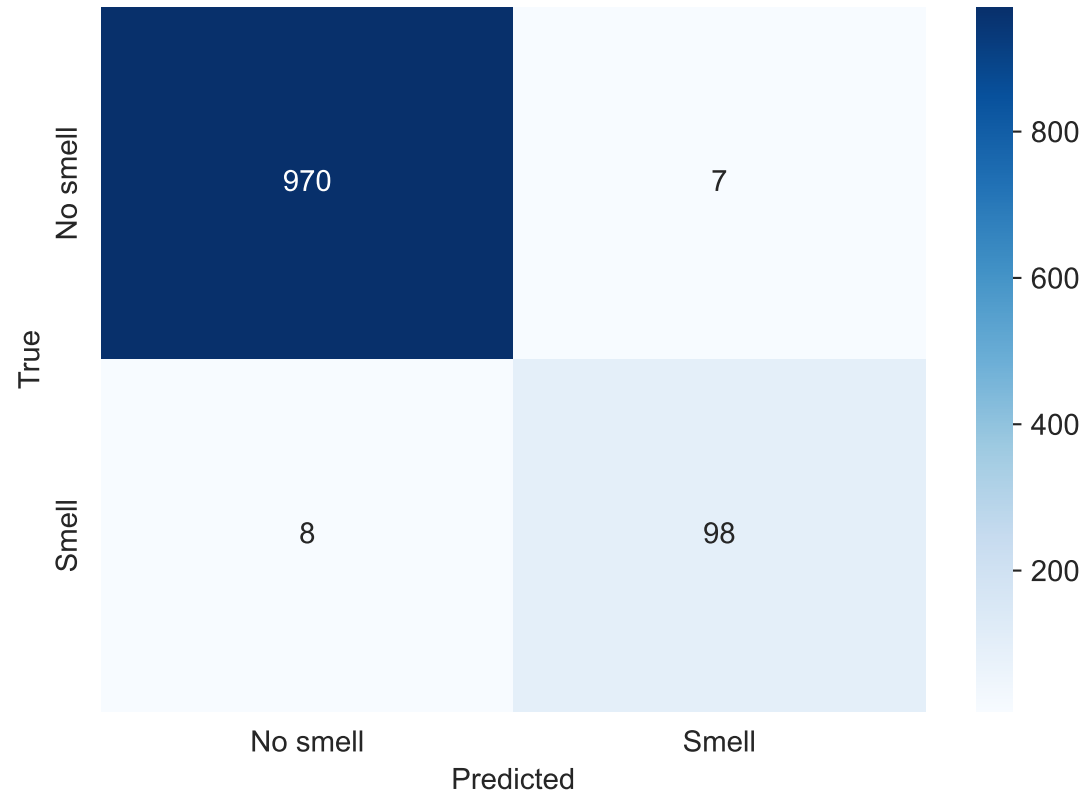
weak_verb (F1=0.929)
