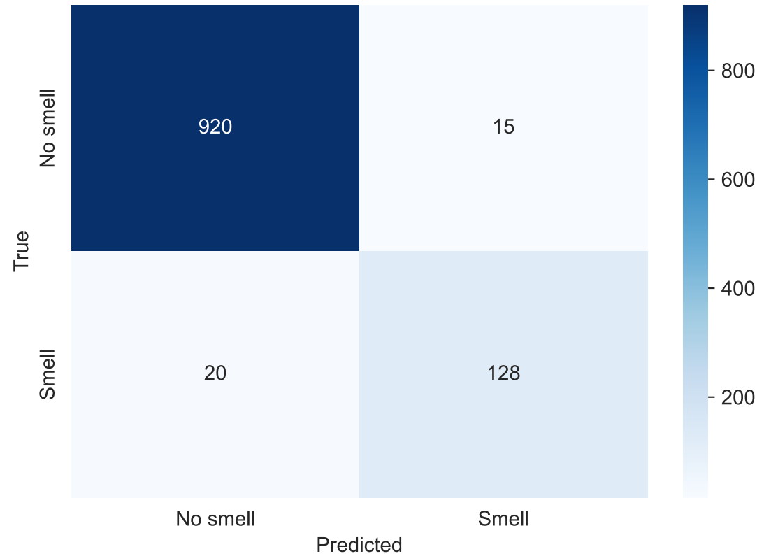
ambiguity (F1=0.880)
