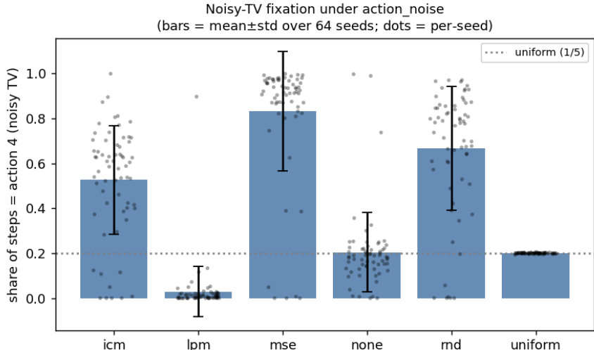
Figure 1: TV-action share under action_noise (bars = mean \pm std; black dots = the 64 per-seed values): fraction of steps spent staring at the noise wall. MSE is trapped on it (0.83); LPM essentially never is (0.03, below even the no-learning baseline); the curiosity baselines RND/ICM are partially fooled; uniform sits at exactly 1/5 (chance). The per-seed dots show the full distribution behind each bar — LPM is a tight mass at \approx 0 , while MSE/RND/ICM spread high (each with a low-tail of lucky seeds), confirming the effect is not a mean-only artifact.
