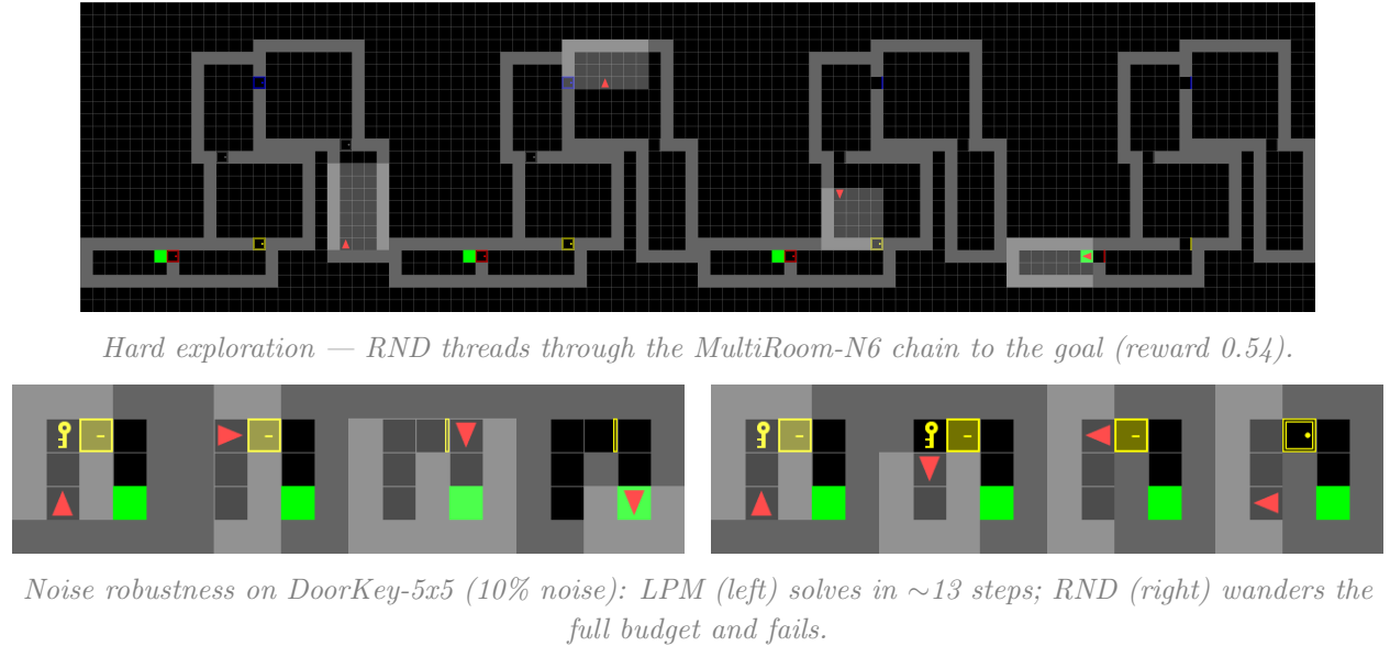
Figure 7: Trajectory film-strips (evenly-spaced frames). Top: intrinsic motivation enables hard exploration. Bottom: LPM is noise-robust where RND is not.
