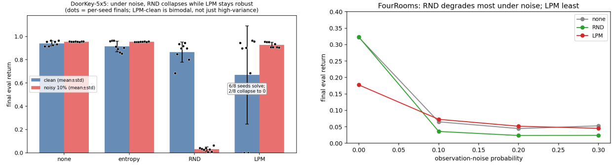
Figure 6: Left: DoorKey-5x5 clean vs. 10% observation noise (bars = mean±std; black dots = the per-seed final returns). RND collapses ( 0.87 \rightarrow 0.03 ). LPM-clean is bimodal — 6/8 seeds solve ( \approx 0.96 ), 2/8 collapse to 0 — so its mean 0.67 and wide \pm std bar reflect a two-mode split, not measurement noise (no seed actually lands near the mean); yet under noise LPM stays robust ( \rightarrow 0.93 ). Right: FourRooms degradation vs. noise probability — RND falls off the most, LPM the least.
