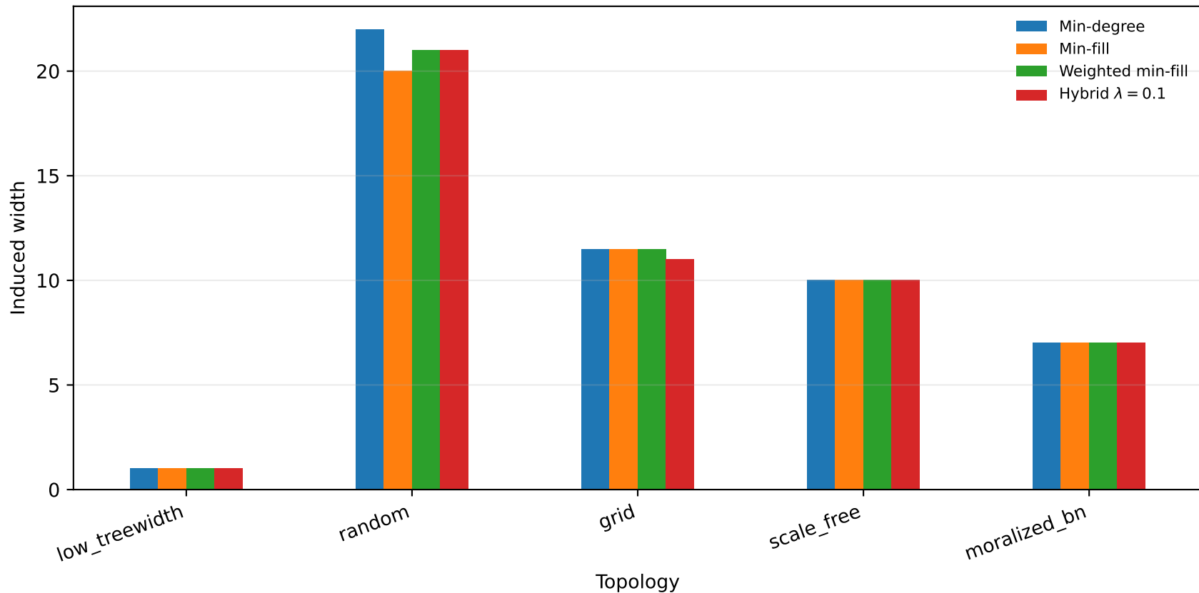
Induced width by topology
