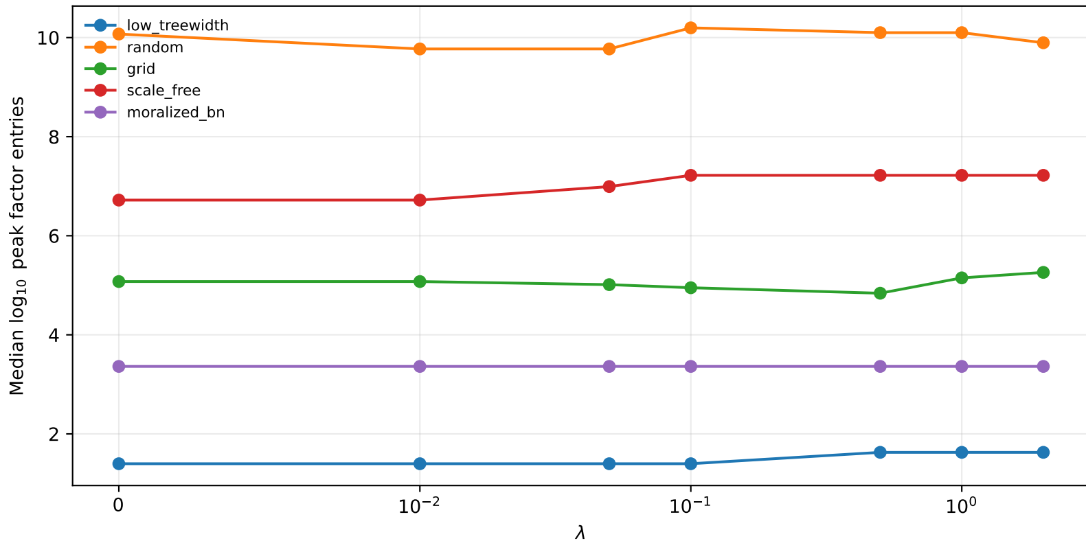
Hybrid lambda sensitivity
