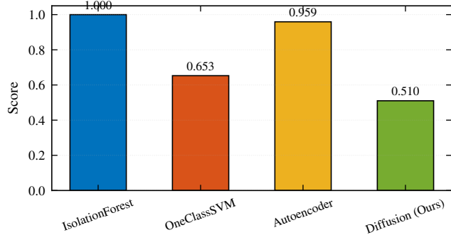
Recall
