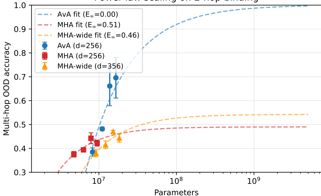
Power-law scaling on 2-hop binding
