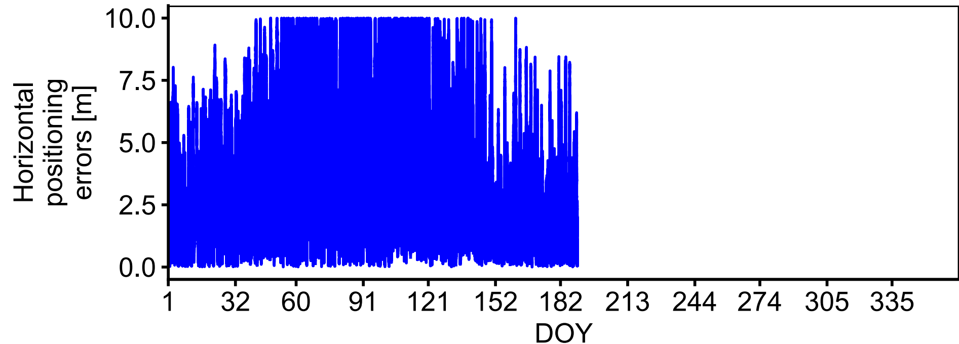
Time series of filtered horizontal positioning errors [m] ( < 10 ) for Darwin, NT, Australia (2014)
