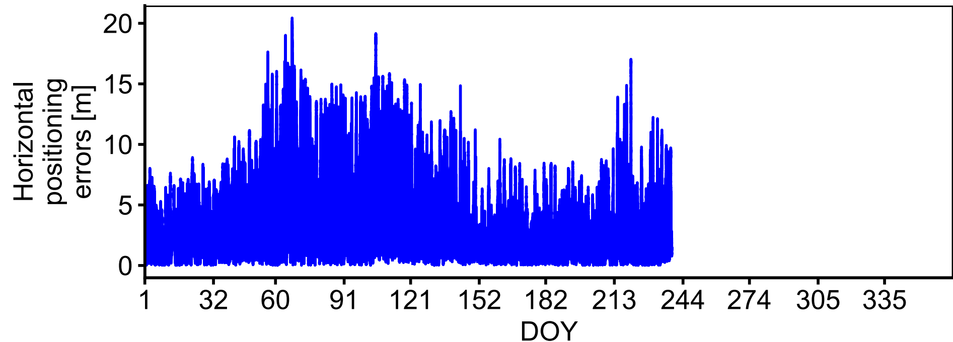
Time series of horizontal positioning errors [m] for Darwin, NT, Australia (2014)
