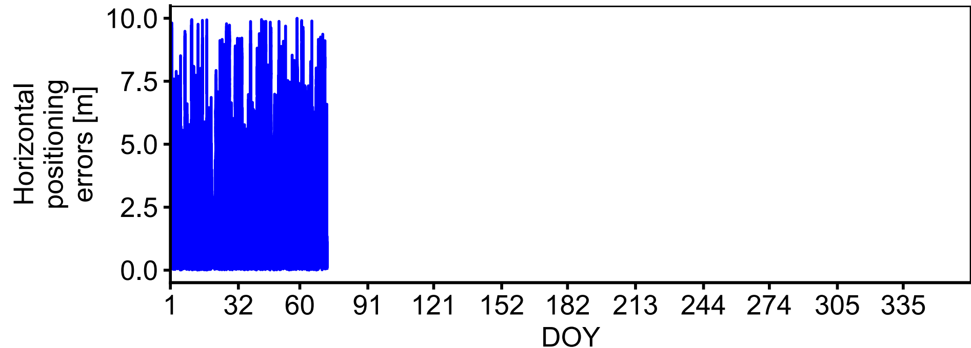
Time series of filtered horizontal positioning errors [m] ( < 10 ) for Iqaluit, NU, Canada (2014)
