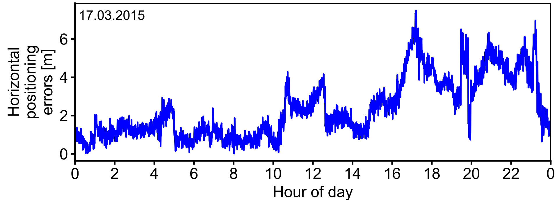
Time series of horizontal positioning errors [m] for storm 1 (17.03.2015)
