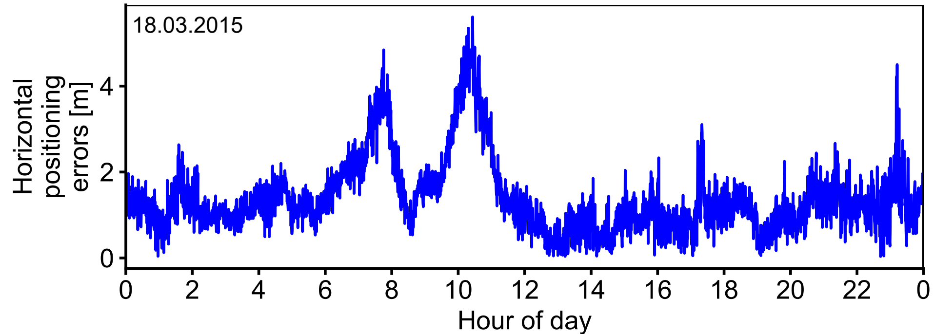
Time series of horizontal positioning errors [m] for storm 1 (18.03.2015)
