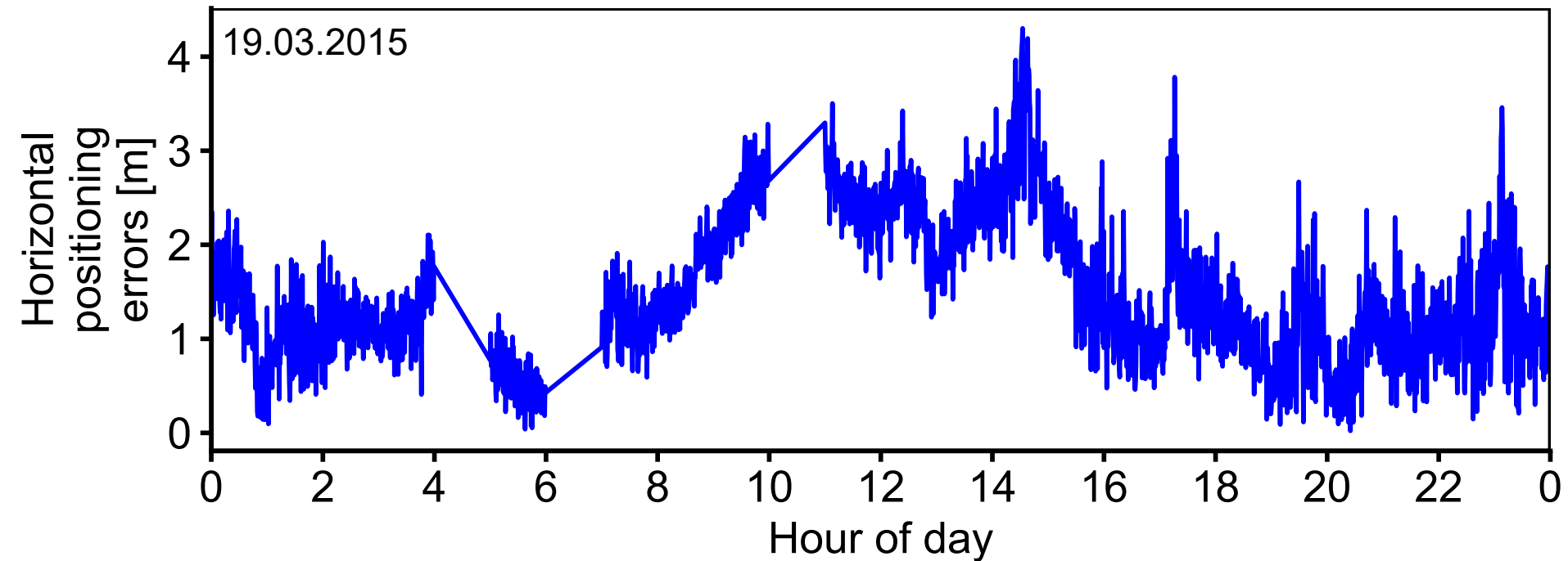
Time series of horizontal positioning errors [m] for storm 1 (19.03.2015)
