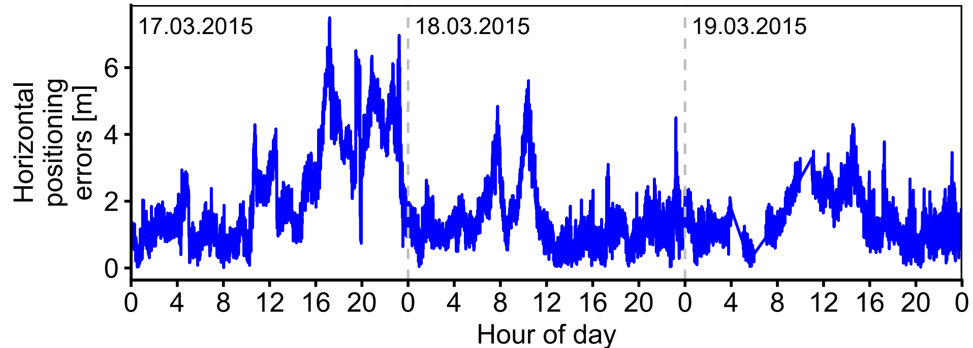
Time series of horizontal positioning errors [m] for storm 1 (17.-19.03.2015)
