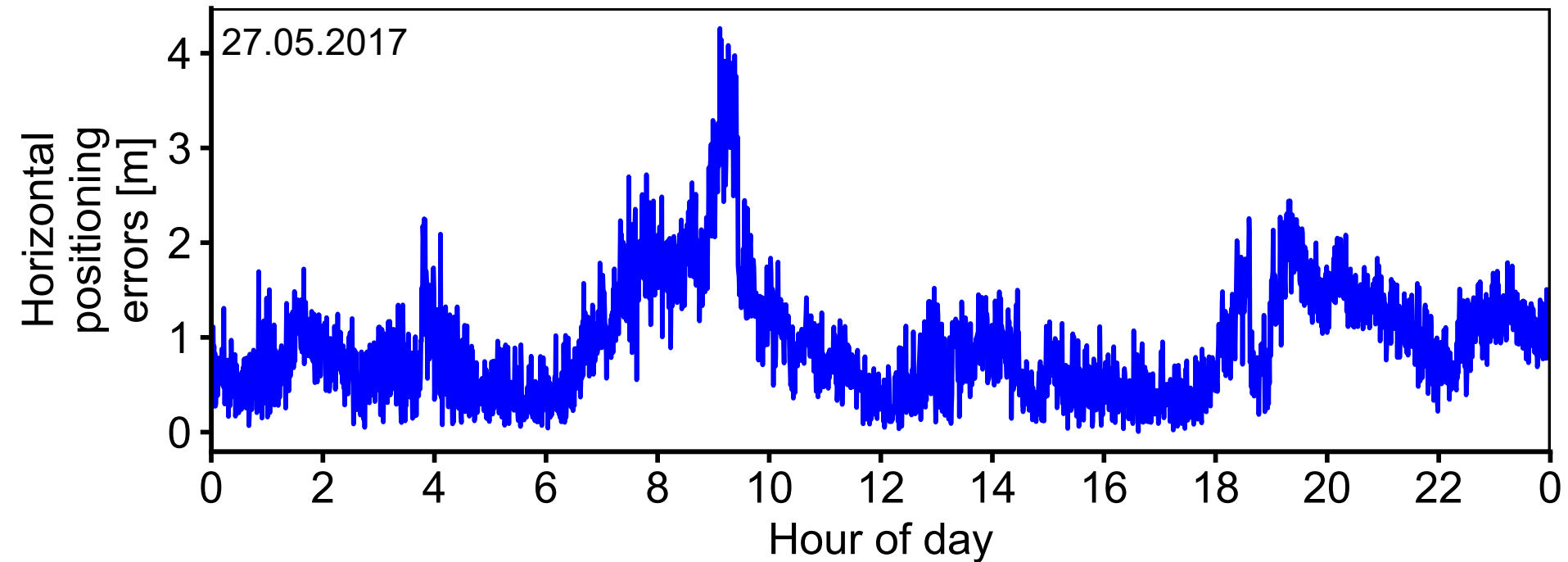
Time series of horizontal positioning errors [m] for storm 2 (27.05.2017)
