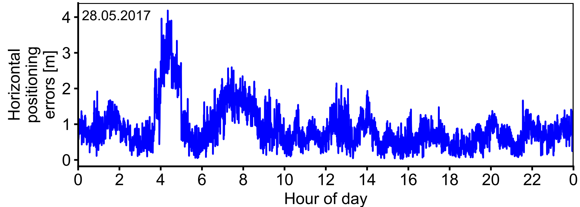
Time series of horizontal positioning errors [m] for storm 2 (28.05.2017)
