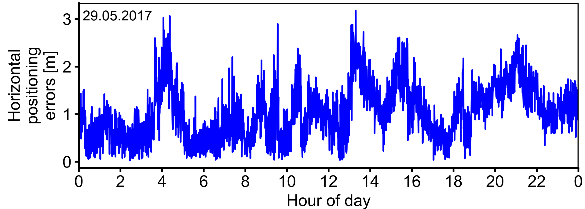
Time series of horizontal positioning errors [m] for storm 2 (29.05.2017)
