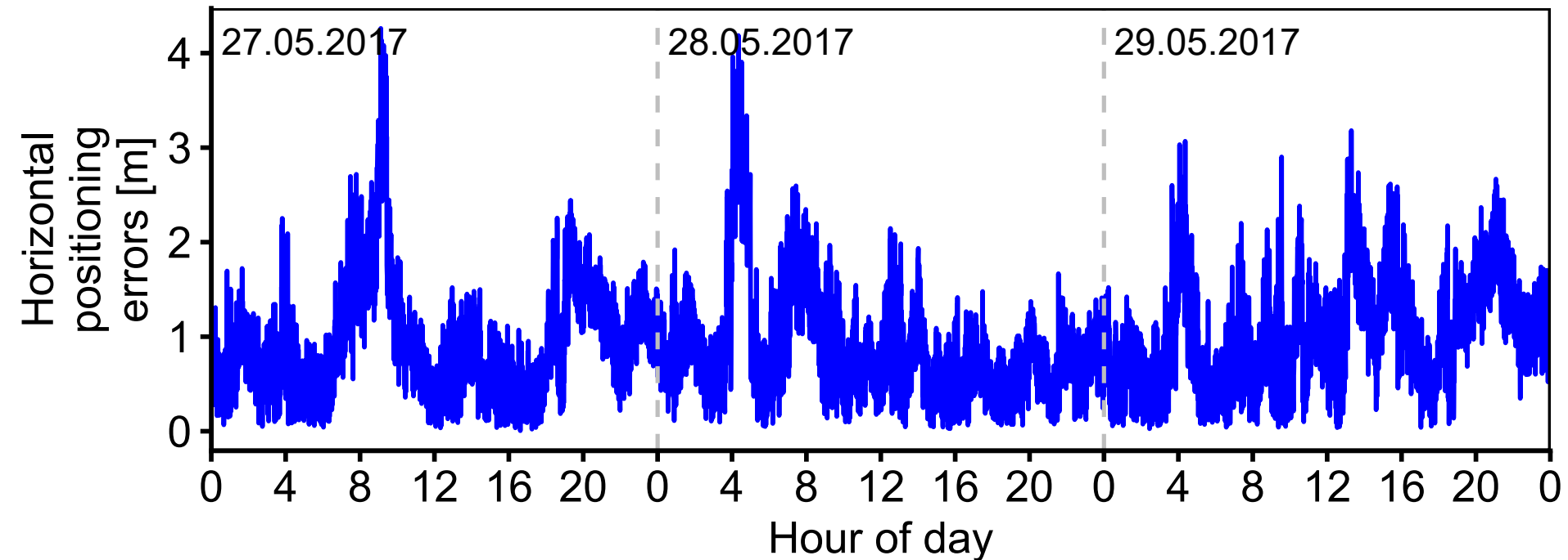
Time series of horizontal positioning errors [m] for storm 2 (27.-29.05.2017)
