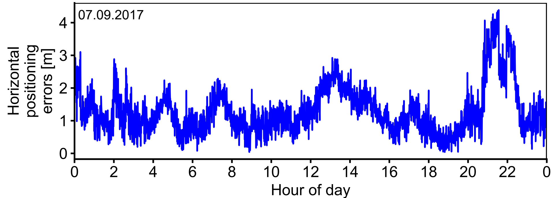
Time series of horizontal positioning errors [m] for storm 3 (07.09.2017)
