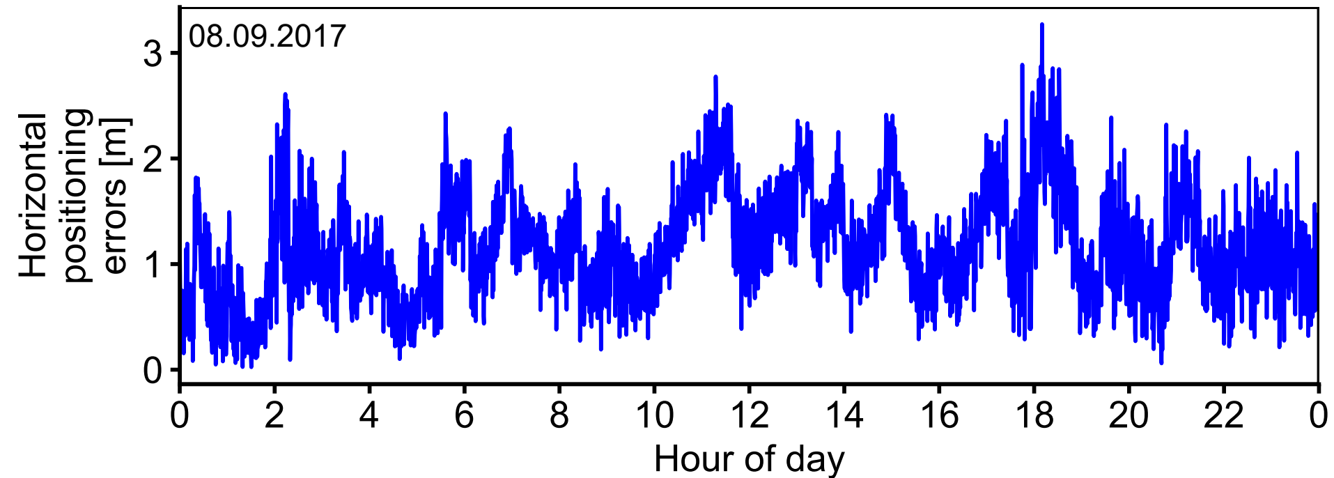
Time series of horizontal positioning errors [m] for storm 3 (08.09.2017)
