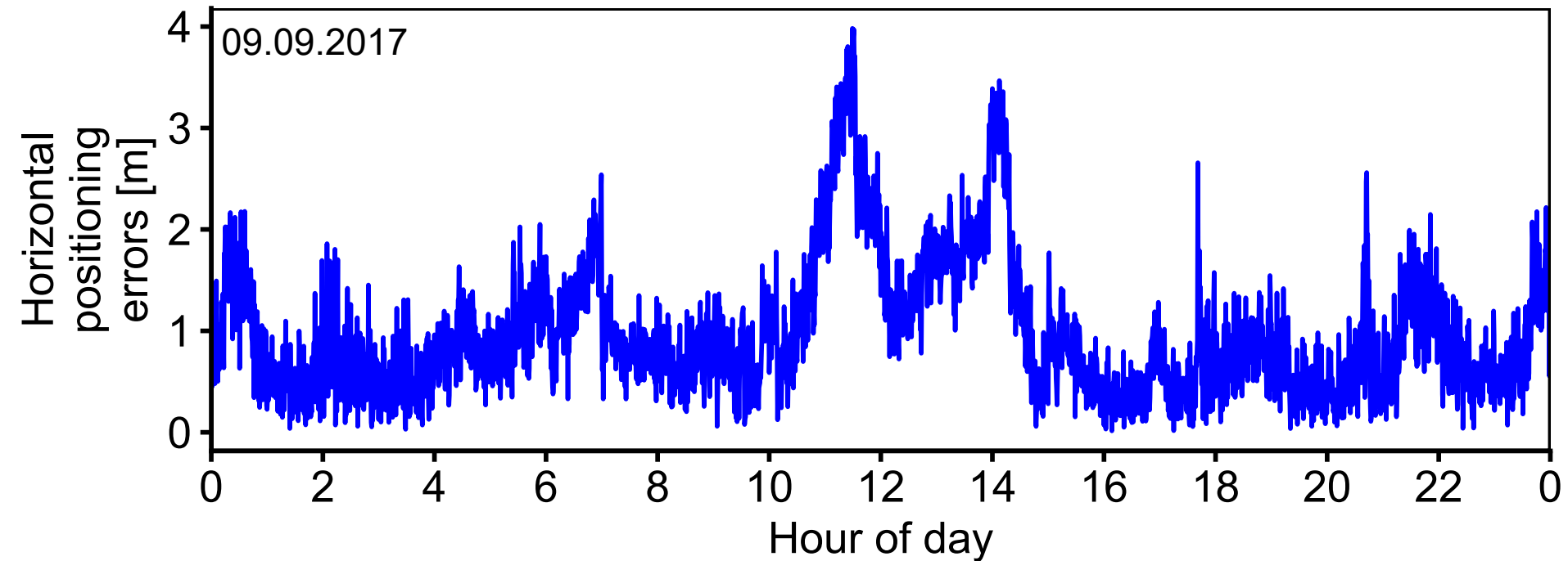
Time series of horizontal positioning errors [m] for storm 3 (09.09.2017)
