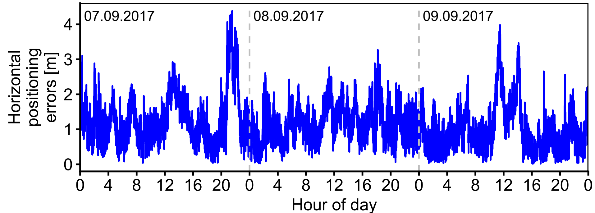
Time series of horizontal positioning errors [m] for storm 3 (07.-09.09.2017)
