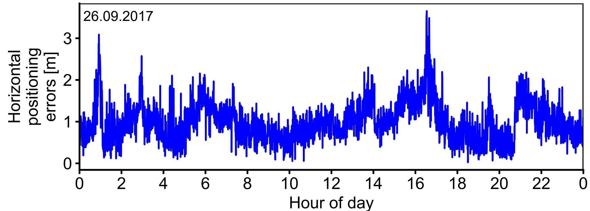
Time series of horizontal positioning errors [m] for storm 4 (26.09.2017)
