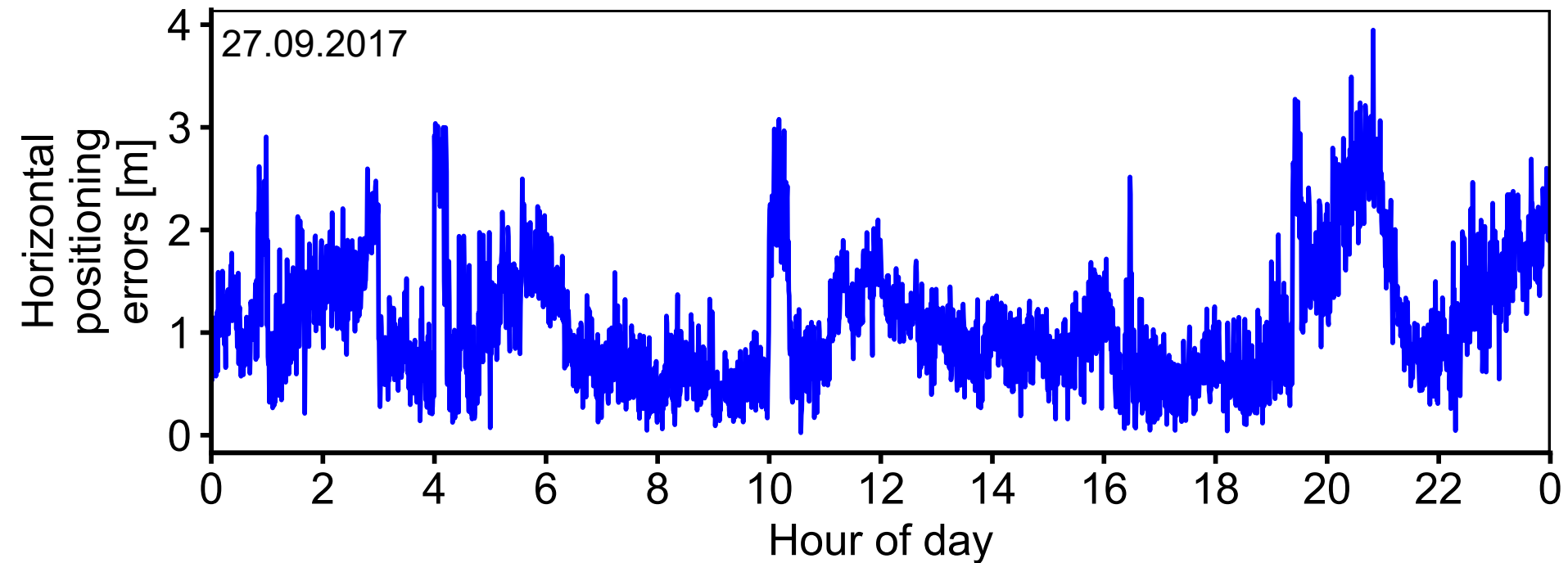
Time series of horizontal positioning errors [m] for storm 4 (27.09.2017)
