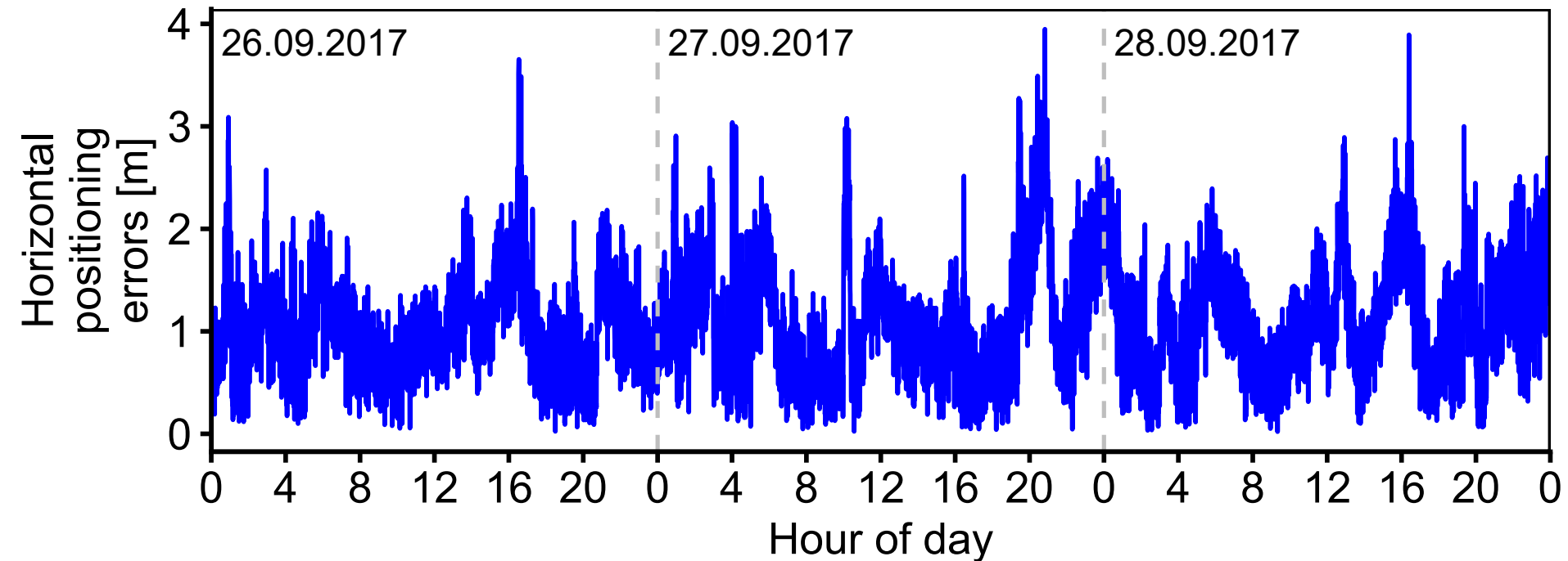
Time series of horizontal positioning errors [m] for storm 4 (26.-28.09.2017)
