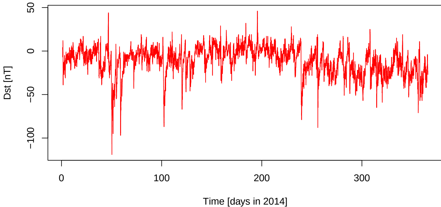
Dst [nT] for days in 2014
