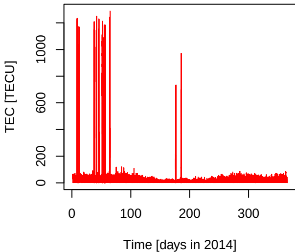
TEC [TECU] for days in 2014
