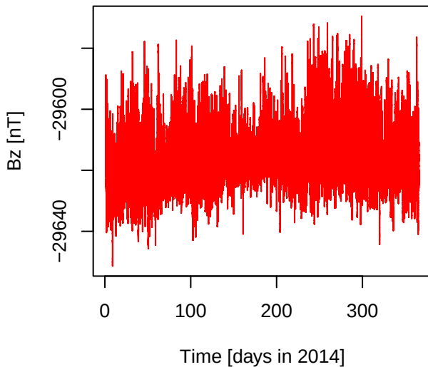
Bz [nT] for days in 2014
