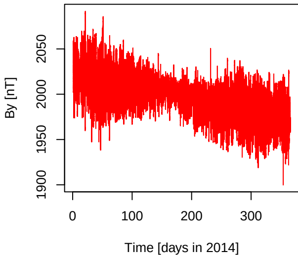
By [nT] for days in 2014
