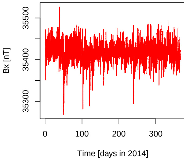
Bx [nT] for days in 2014
