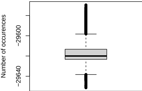
Number of occurrences Bz [nT]
