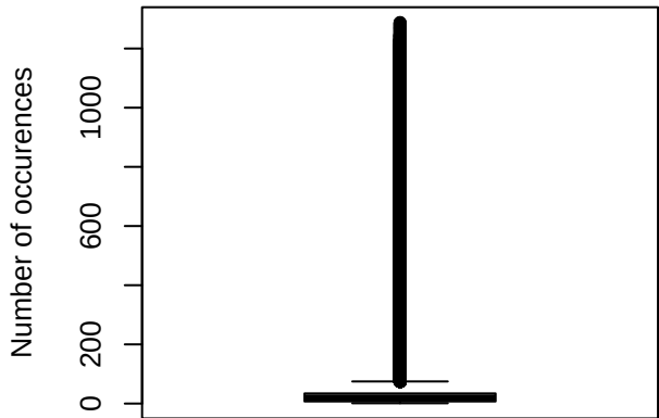
Number of occurrences TEC [TECU]
