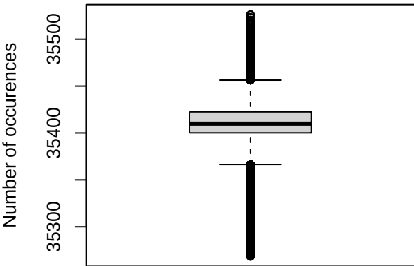
Number of occurrences Bx [nT]
