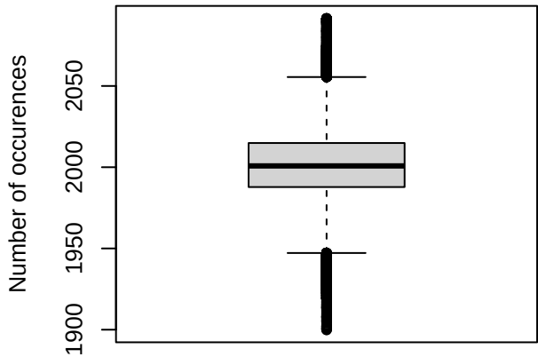
Number of occurrences By [nT]
