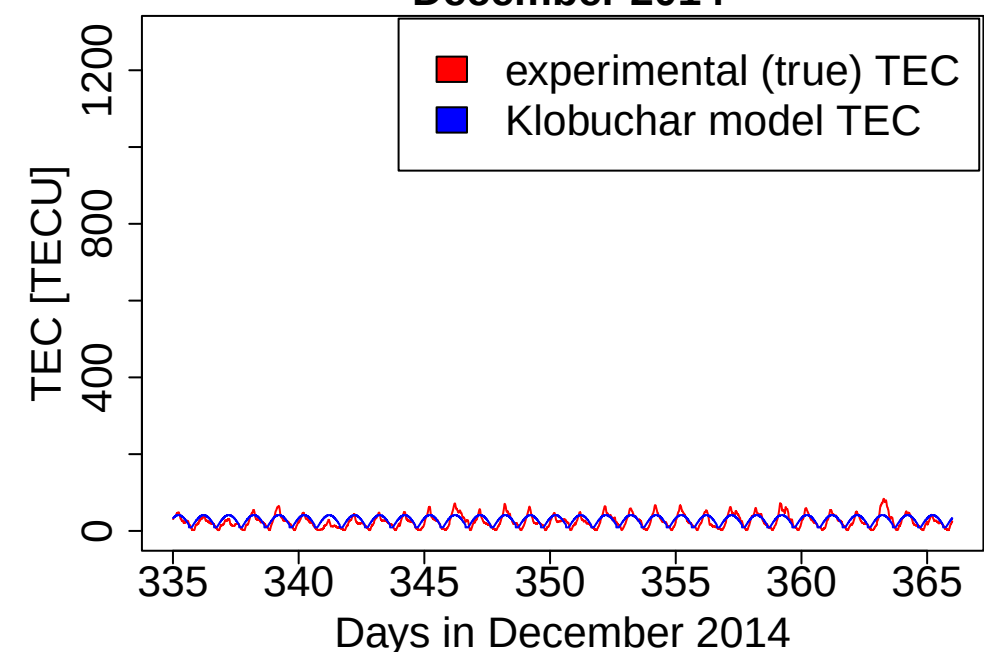
Klobuchar model and experimental (true) TEC December 2014
