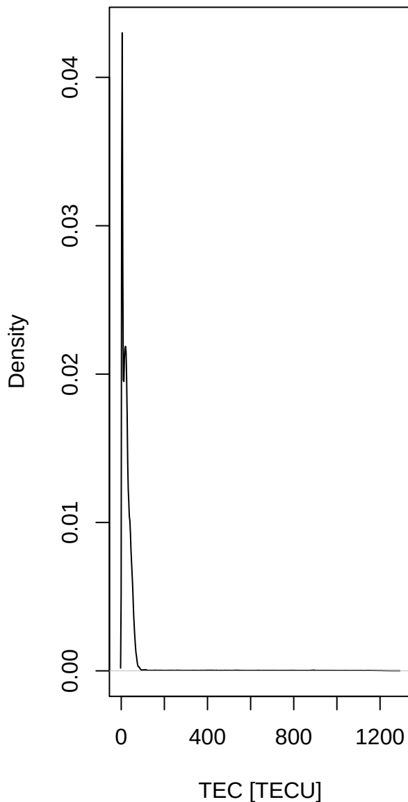
Probability density TEC [TECU]
