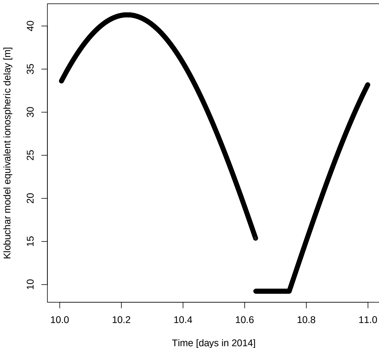
Klobuchar model equivalent ionospheric delay [m] for DOY 10 in 2014
