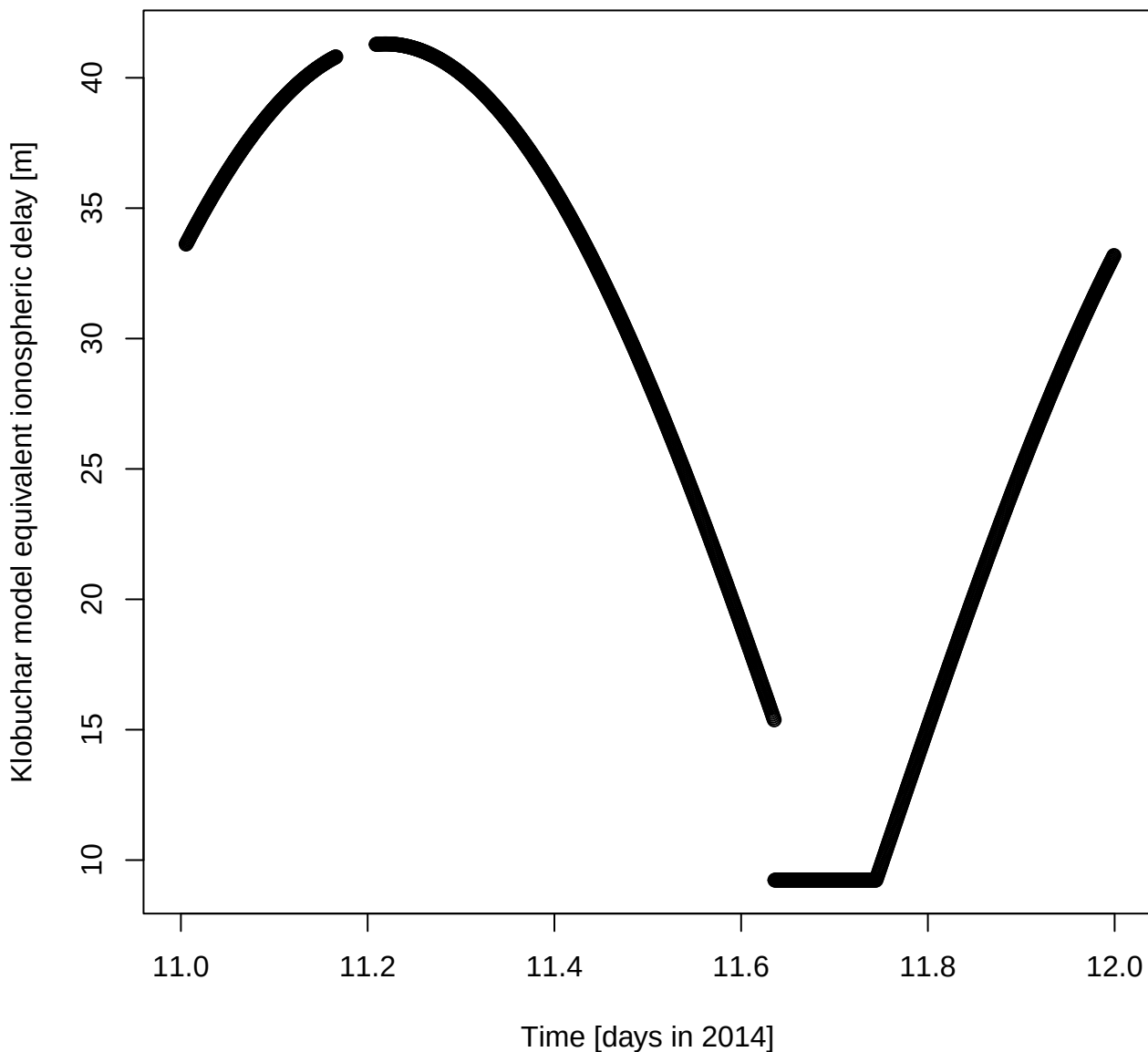
Klobuchar model equivalent ionospheric delay [m] for DOY 11 in 2014
