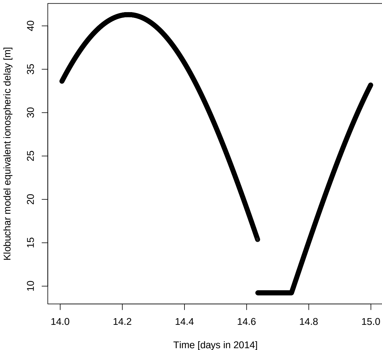
Klobuchar model equivalent ionospheric delay [m] for DOY 14 in 2014
