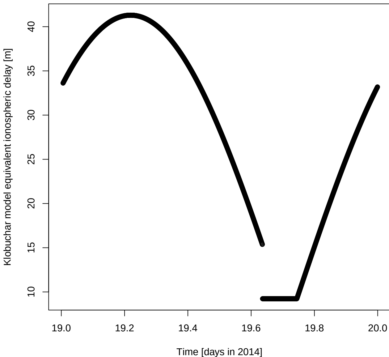
Klobuchar model equivalent ionospheric delay [m] for DOY 19 in 2014
