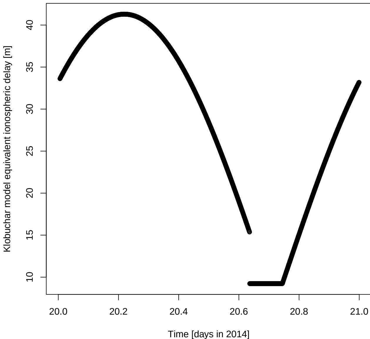
Klobuchar model equivalent ionospheric delay [m] for DOY 20 in 2014
