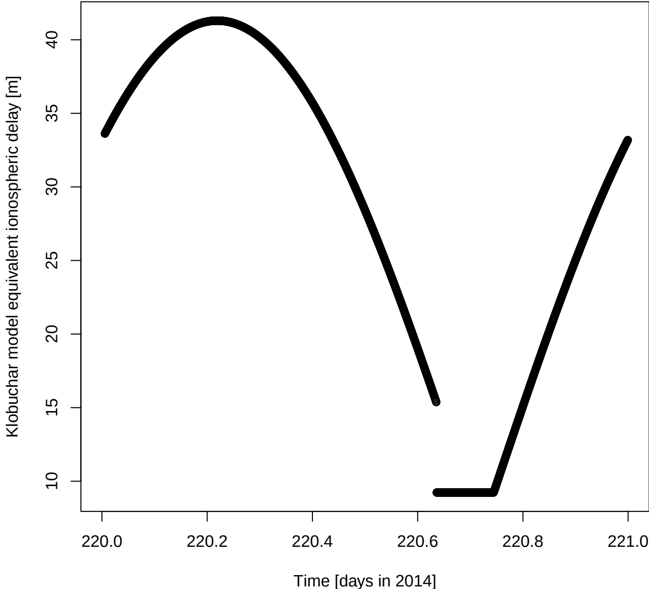
Klobuchar model equivalent ionospheric delay [m] for DOY 220 in 2014
