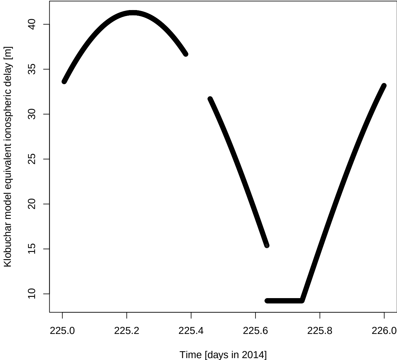
Klobuchar model equivalent ionospheric delay [m] for DOY 225 in 2014
