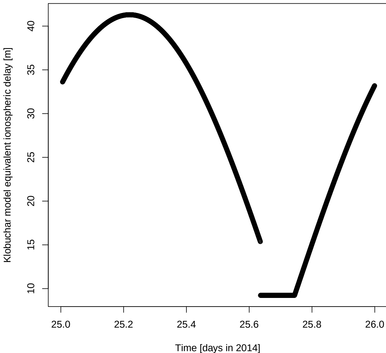
Klobuchar model equivalent ionospheric delay [m] for DOY 25 in 2014
