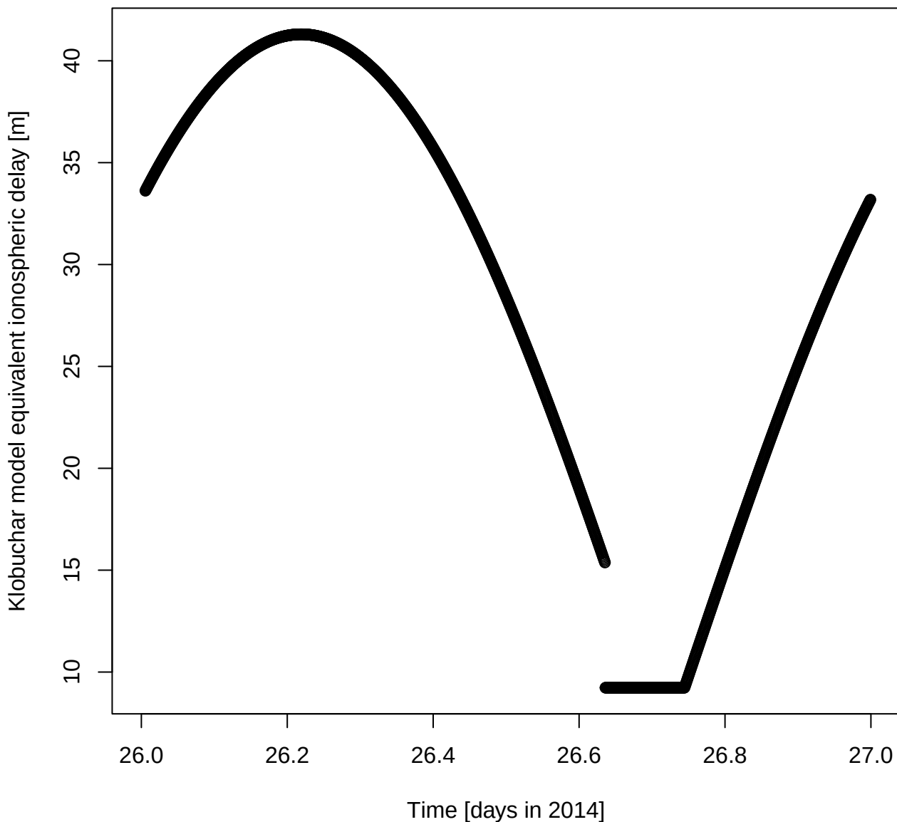
Klobuchar model equivalent ionospheric delay [m] for DOY 26 in 2014
