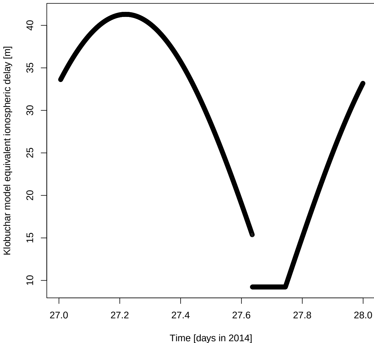
Klobuchar model equivalent ionospheric delay [m] for DOY 27 in 2014
