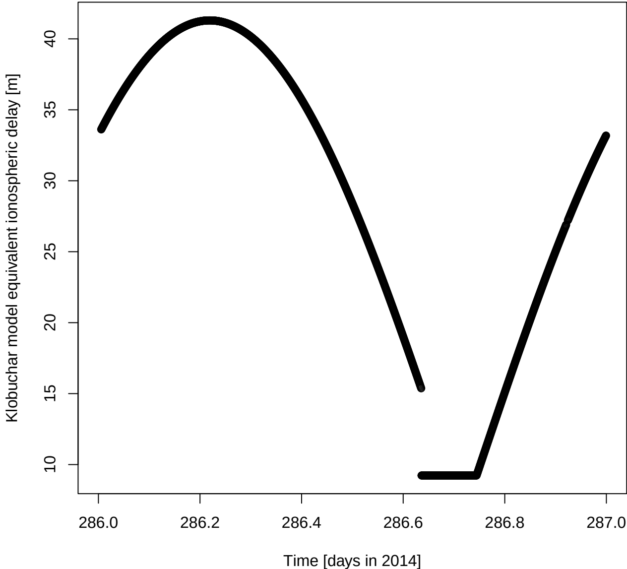
Klobuchar model equivalent ionospheric delay [m] for DOY 286 in 2014
