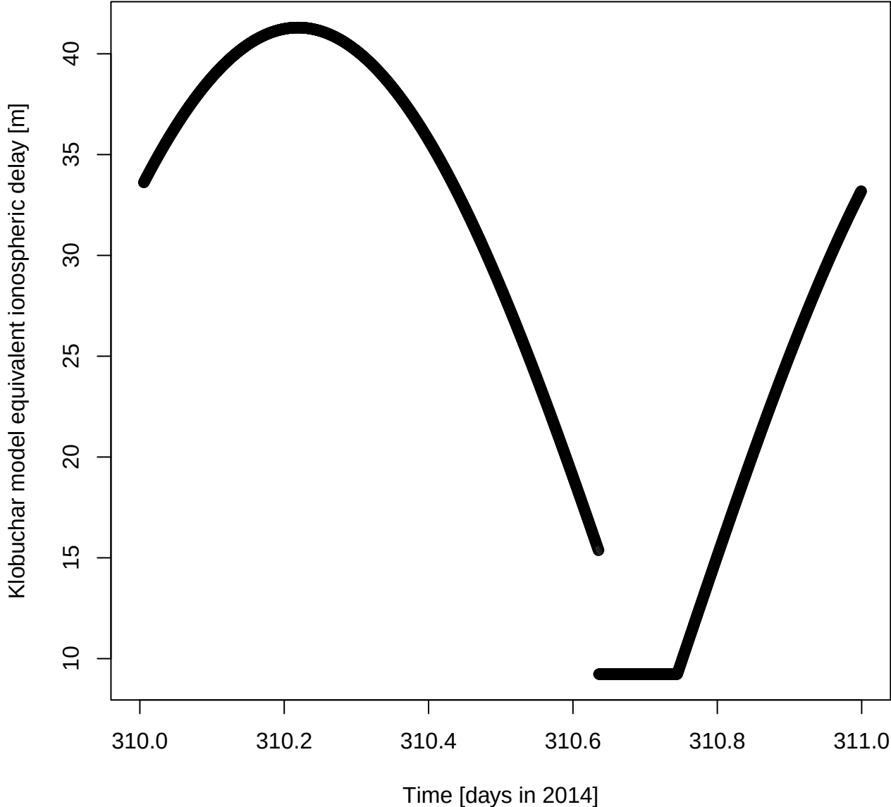
Klobuchar model equivalent ionospheric delay [m] for DOY 310 in 2014
