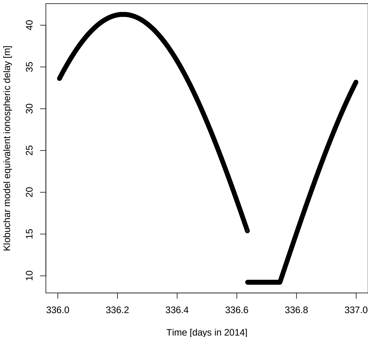
Klobuchar model equivalent ionospheric delay [m] for DOY 336 in 2014
