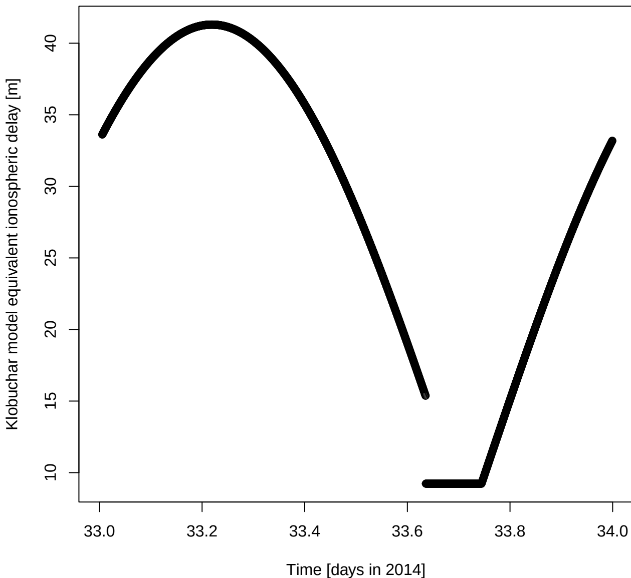
Klobuchar model equivalent ionospheric delay [m] for DOY 33 in 2014
