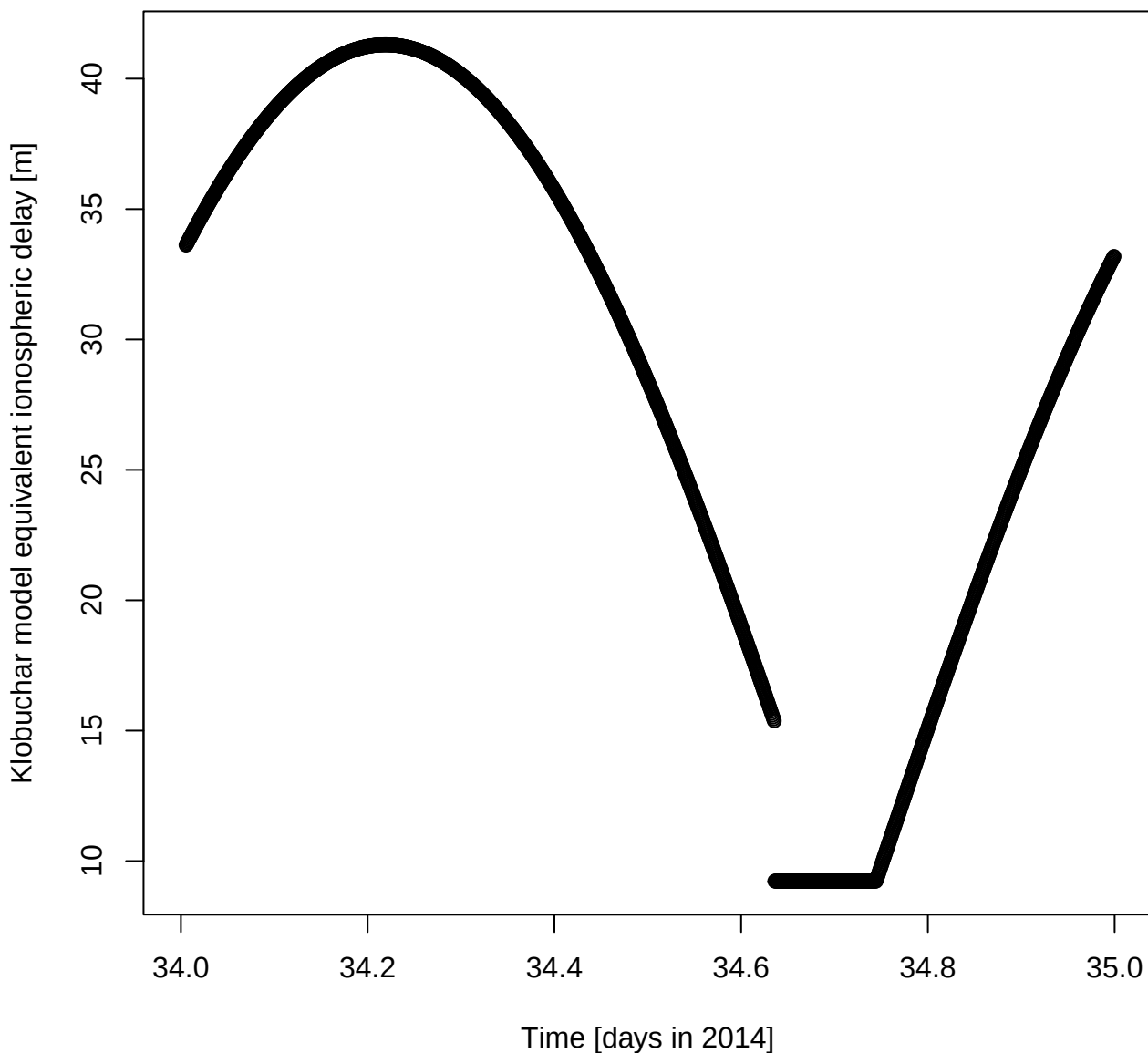
Klobuchar model equivalent ionospheric delay [m] for DOY 34 in 2014
