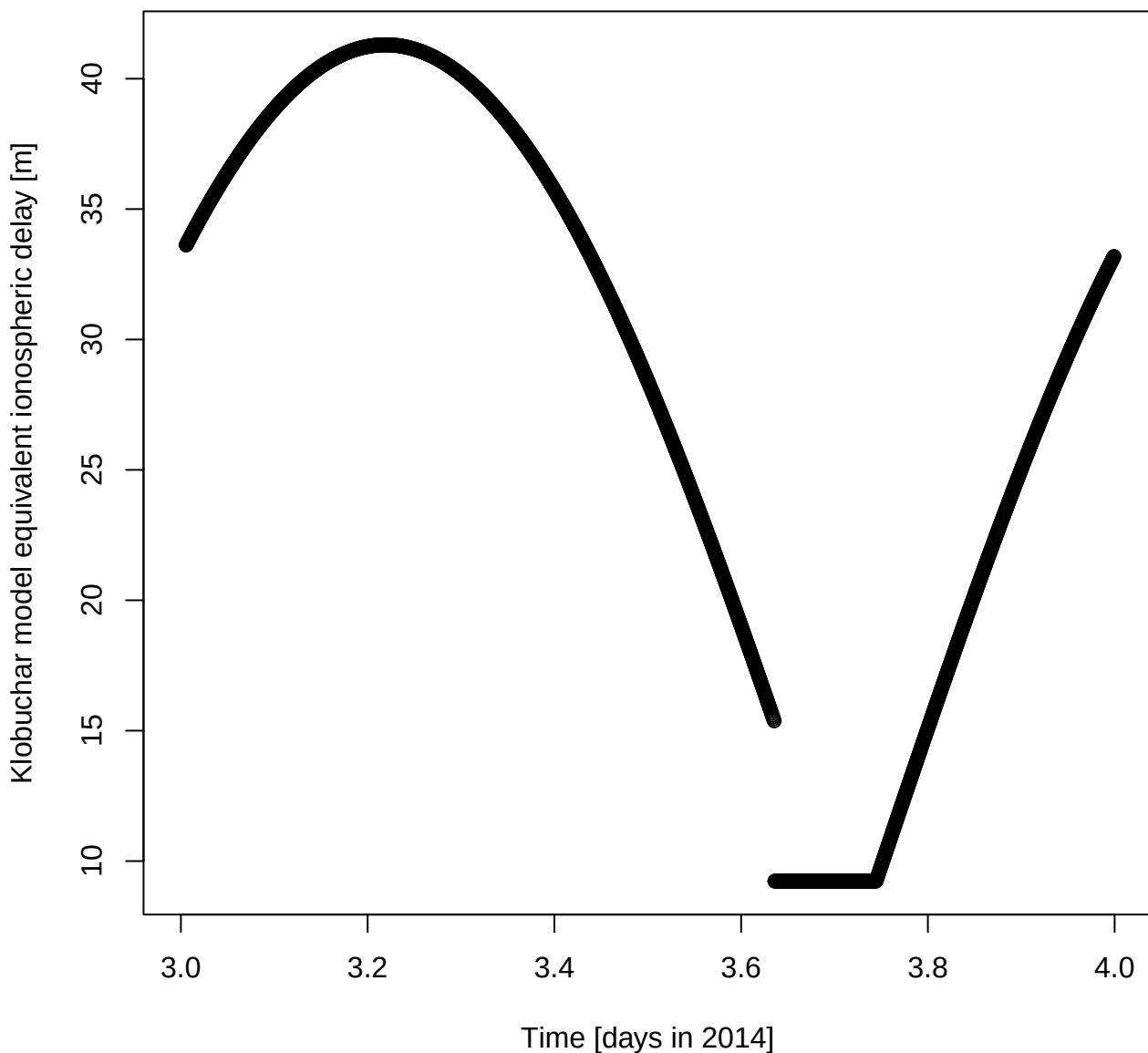
Klobuchar model equivalent ionospheric delay [m] for DOY 3 in 2014
