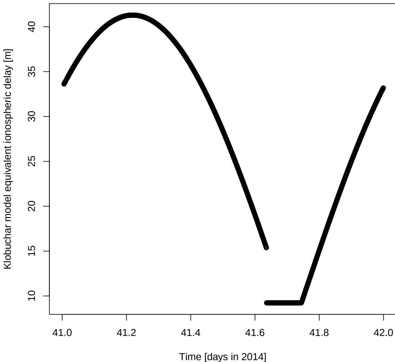
Klobuchar model equivalent ionospheric delay [m] for DOY 41 in 2014
