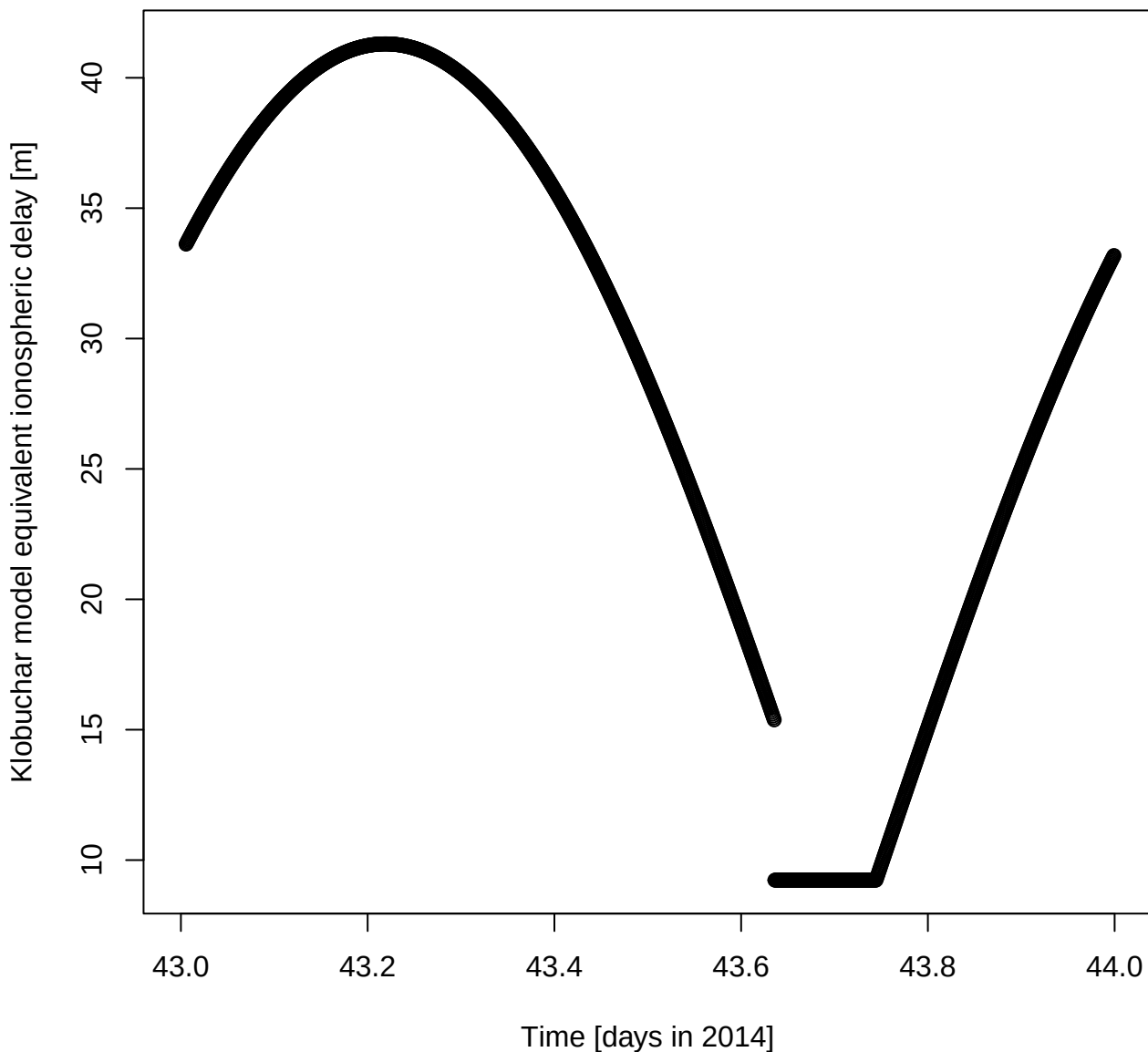
Klobuchar model equivalent ionospheric delay [m] for DOY 43 in 2014
