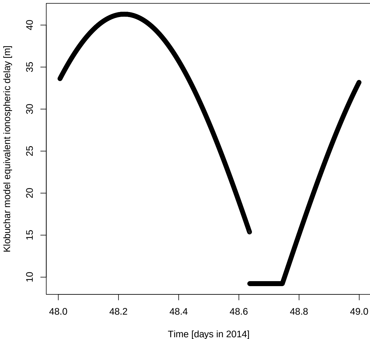
Klobuchar model equivalent ionospheric delay [m] for DOY 48 in 2014
