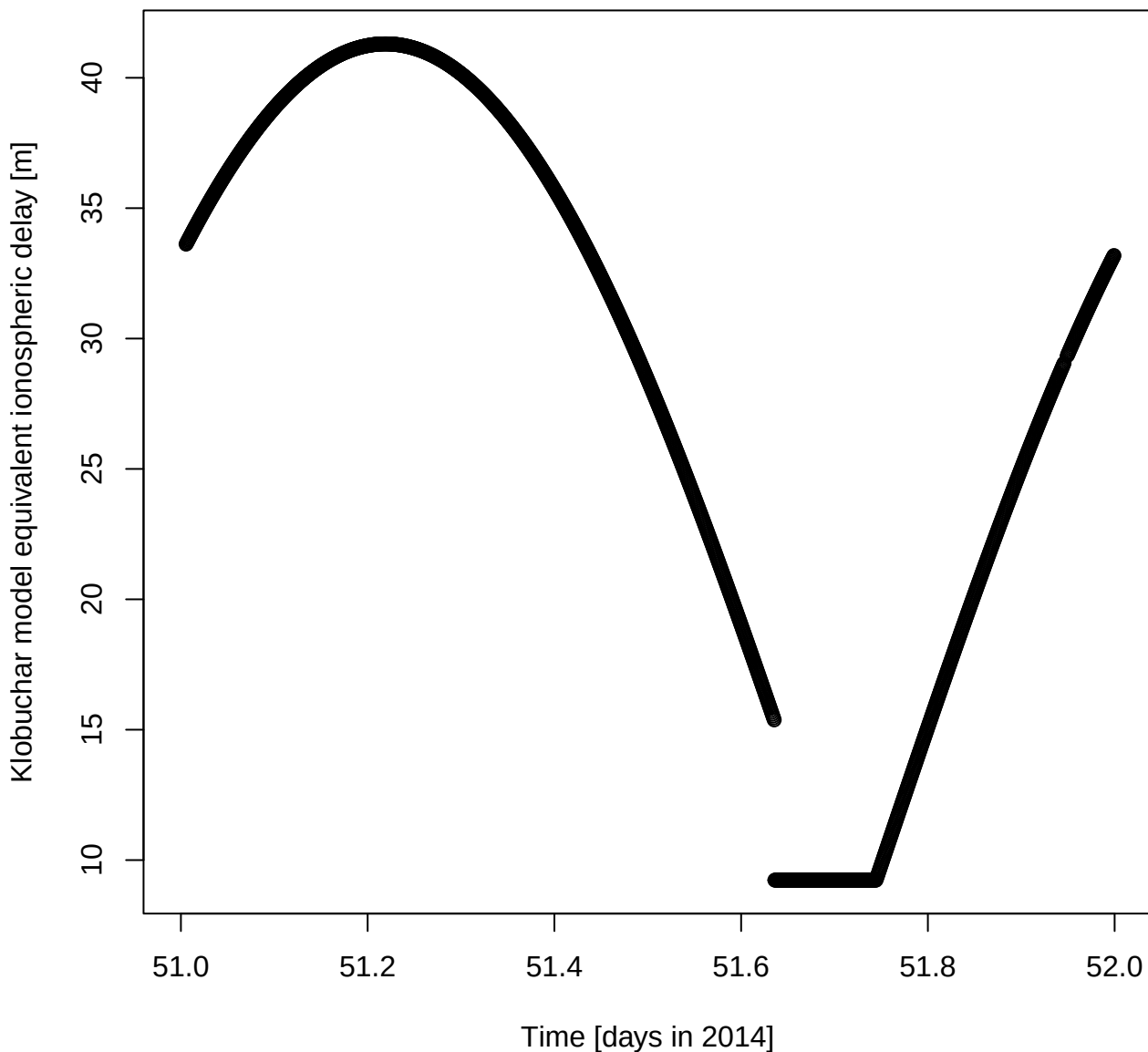
Klobuchar model equivalent ionospheric delay [m] for DOY 51 in 2014
